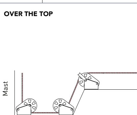
SINGLE LINE REEFING
