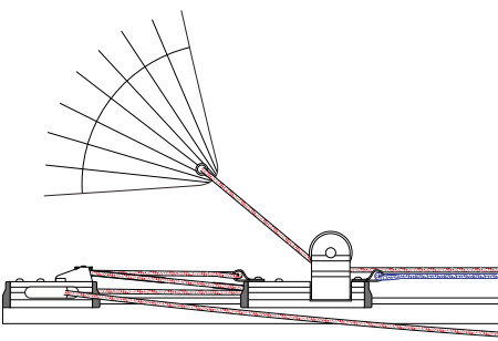
HALYARD LED AFT
