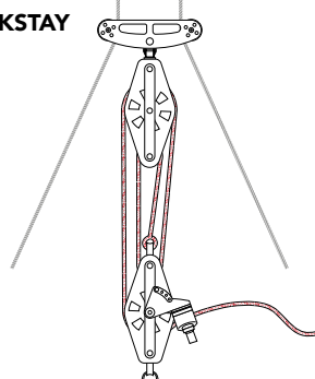
8:1 SPLIT BACKSTAY
