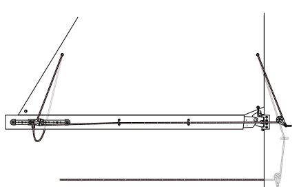
SINGLE LINE REEFING
