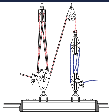
16:1 SPLIT BACKSTAY
