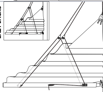
LAZY JACKS
