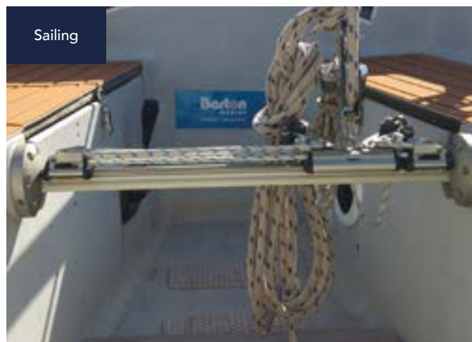
Removable mainsheet track system kits create more space in the cockpit.
