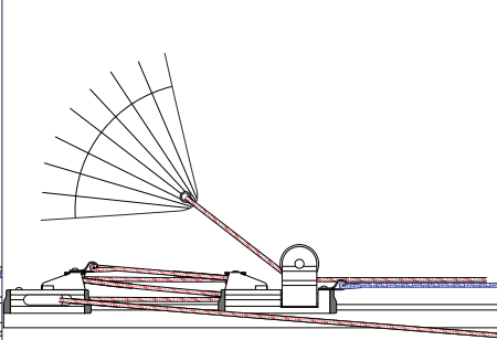
WINCH DECK ORGANISER
