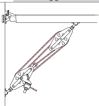
8:1 CASCADED KICKER
