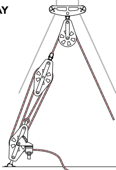
16:1 SPLIT BACKSTAY
