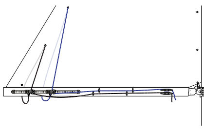
SLAB REEF
